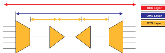
Figure 4: OTN layer structure; as with SONET/SDH, the OTN has a layered structure design
