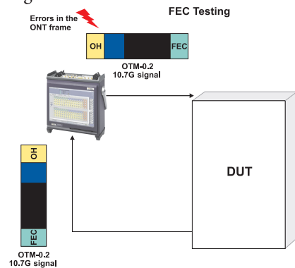
Figure 22: FEC test setup
