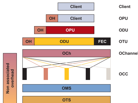
Figure 5: Basic OTN transport structure
