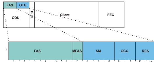
Figure 7: Frame alignment and OTU OH structure
