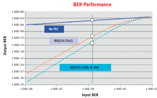
Figure 18: Effect of using FEC with various algorithms
