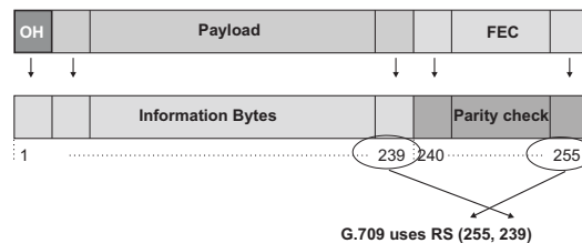
Figure 17: Forming of parity check
