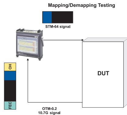
Figure 21: Conducting mapping and demapping tests
