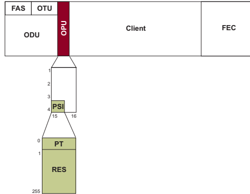
Figure 10: Overhead of OPU
