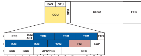
Figure 11: Overhead structure of ODU
