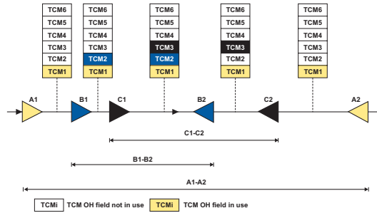
Figure 13: Possible TCM structure in an OTN
