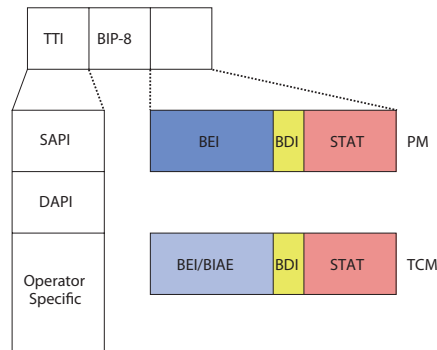
Figure 12: TCM and PM overhead structures
