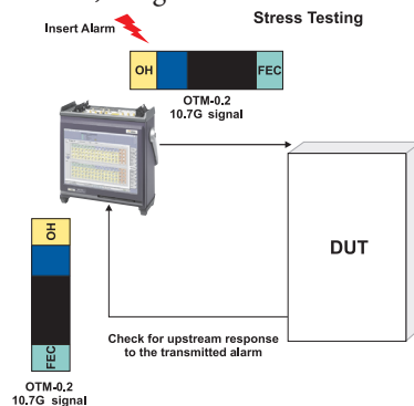
Figure 20: Setup for stimulus testing
